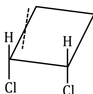
Plane of symmetry
