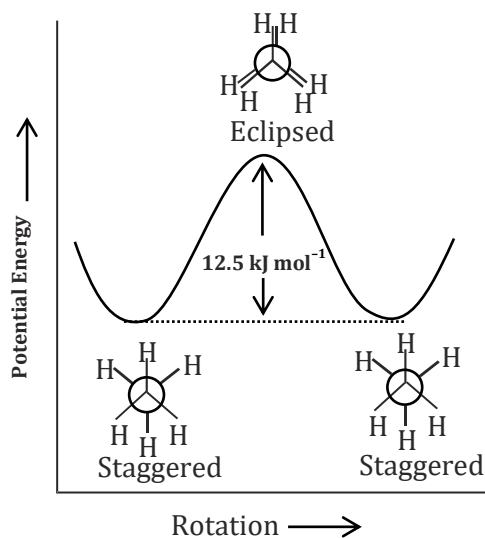
Changes in energy during rotation about C-C bond in
