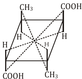
Centre of symmetry
